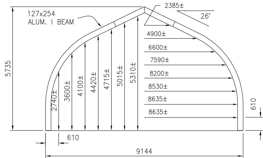
SECTION 9.1m STRUCTURE 1:100
