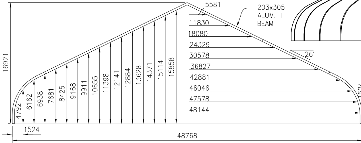
○ SECTION 48.8m STRUCTURE (CLEARANCES) 1:300
