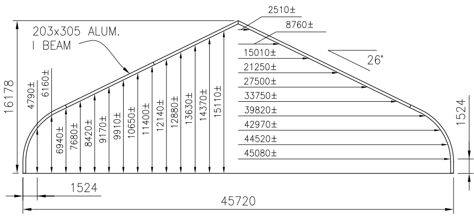
SECTION 45.7m STRUCTURE 1:400
