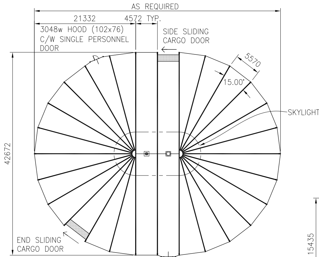
PLAN VIEW 1:500
