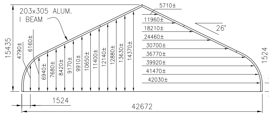
SECTION 42.7m STRUCTURE 1:400
