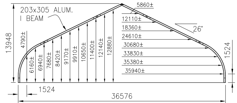
SECTION 36.6m STRUCTURE 1:400
