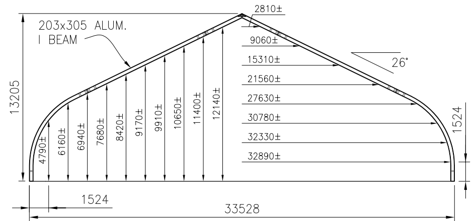
○ SECTION 33.5m STRUCTURE 1:300
