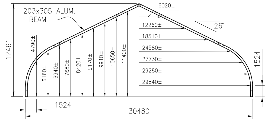
SECTION 30.5m STRUCTURE 1:300
