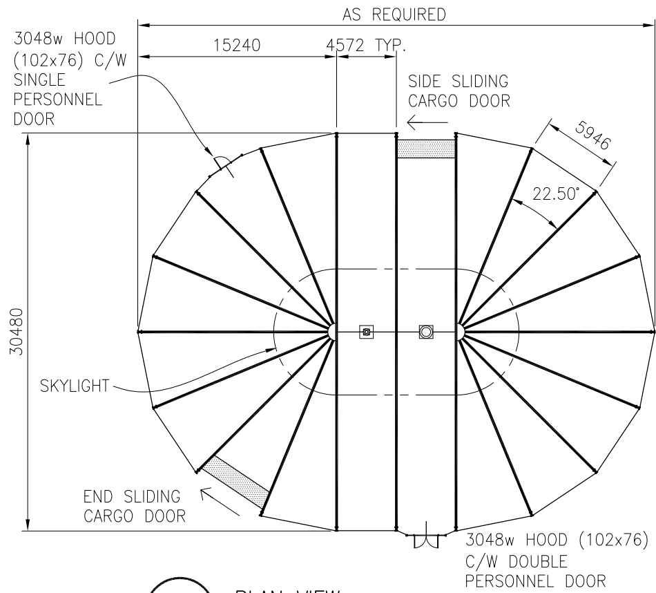
PLAN VIEW 1:400
