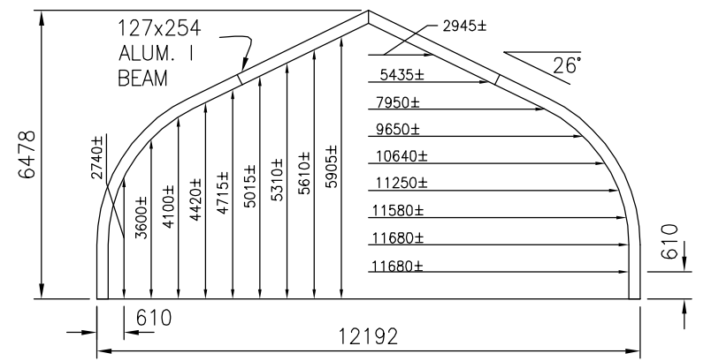
SECTION 12.2m STRUCTURE 1:150
